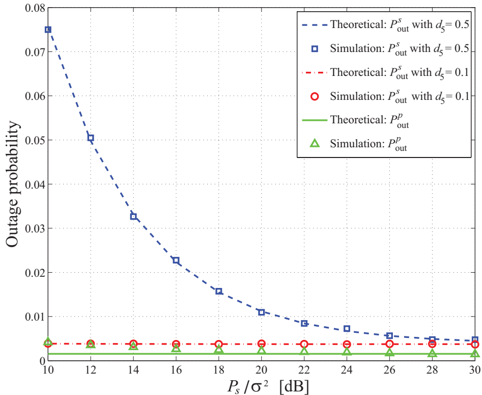
Figure 5.6. Outage probability for various values of P_s / \sigma^2 .
