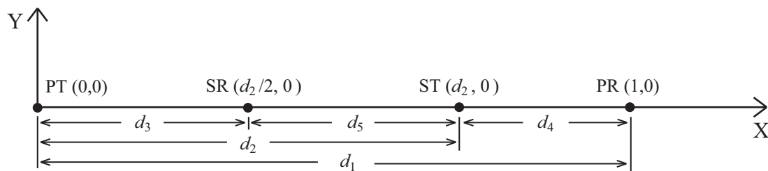
Figure 5.4. Locations of primary and secondary terminals.
