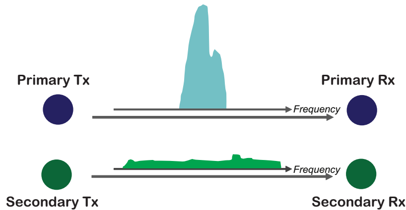
Figure 1.3. Underlay CR with UWB.
